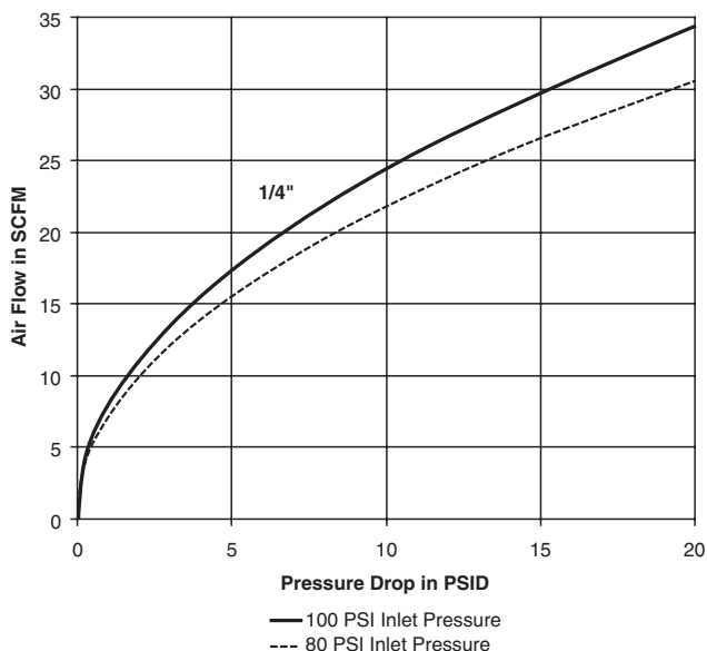
UC Series Coupler (1/4" sizeZ)
